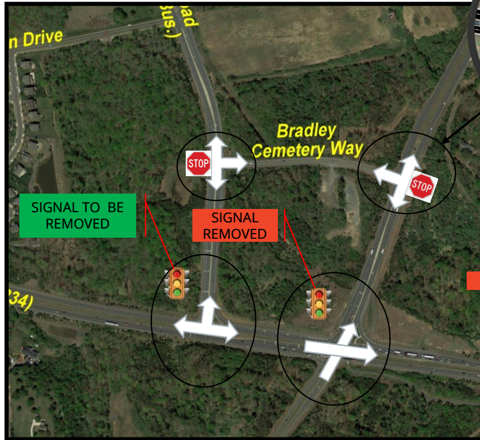
Existing Intersection (Route 234 – Brentsville Road)
