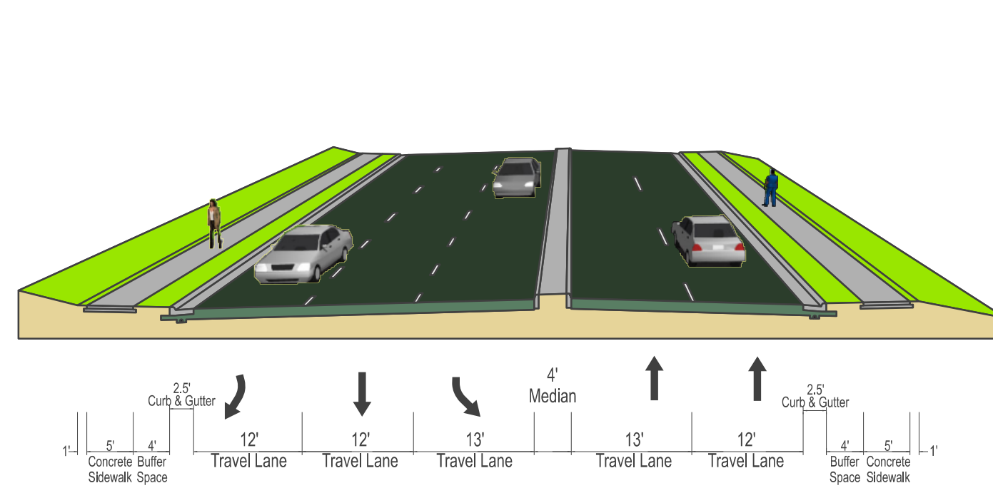
Typical Section Graham Park Road (East of Route 1)
