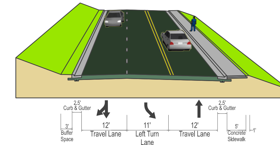
Typical Section Graham Park Road (West of Route 1)
