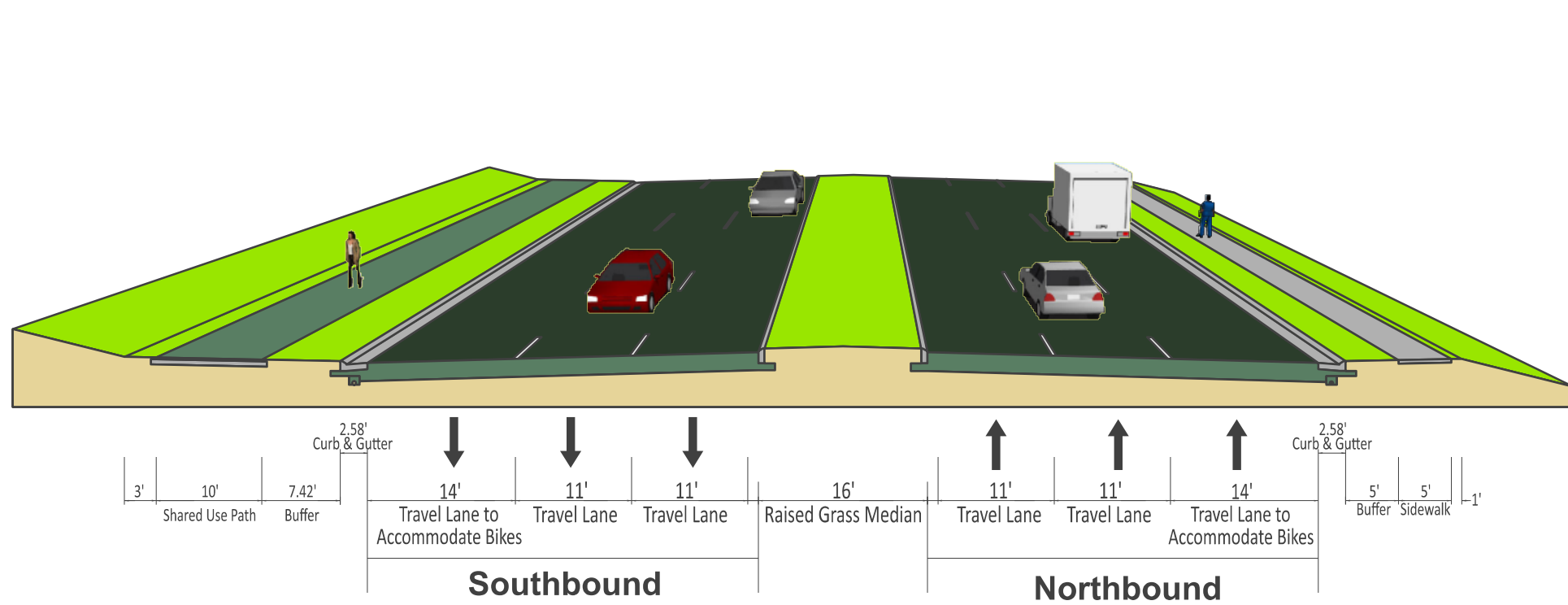
Typical Section Route 1/Fraley Boulevard
